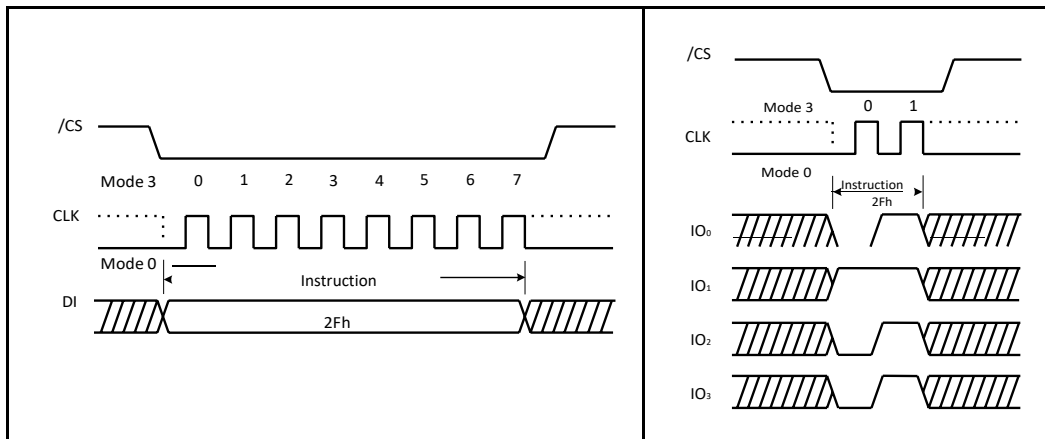
Figure 43. Write Security Register instruction for SPI Mode (left) and QPI Mode (right)
