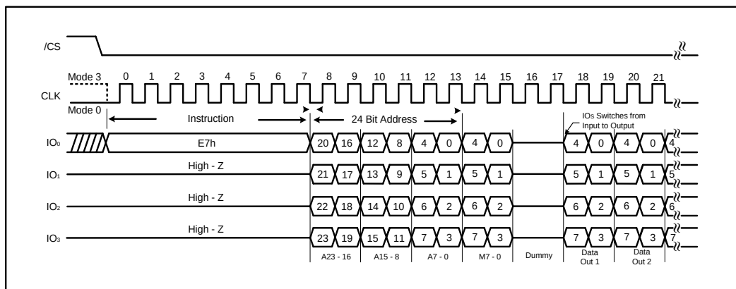
Figure 34a. Word Read Quad I/O instruction (Initial instruction or previous set M7-0 ≠ Axx, SPI Mode)
