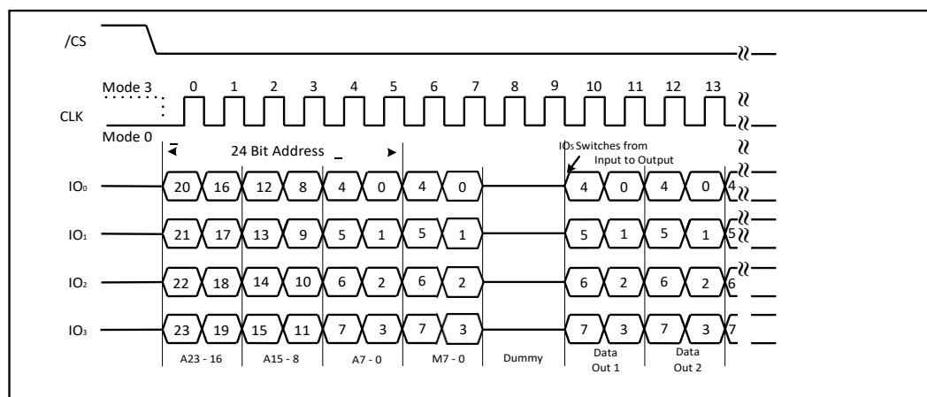
Figure 34b. Word Read Quad I/O instruction (Previous instruction set M7-0= Axh, SPI Mode)
