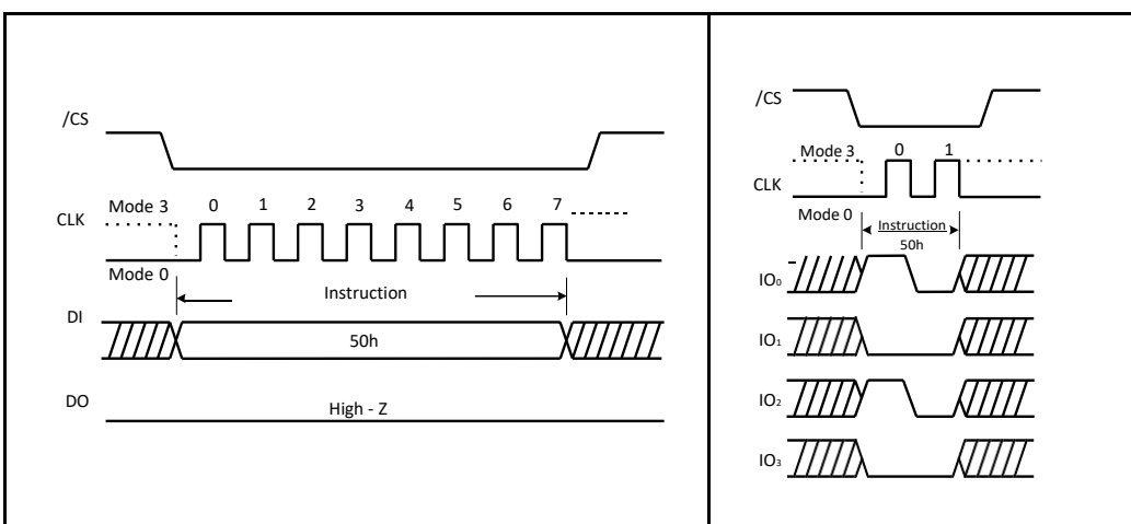
Figure 7. Write Enable for Volatile Status Register Instruction for SPI Mode (left) and QPI Mode (right)
