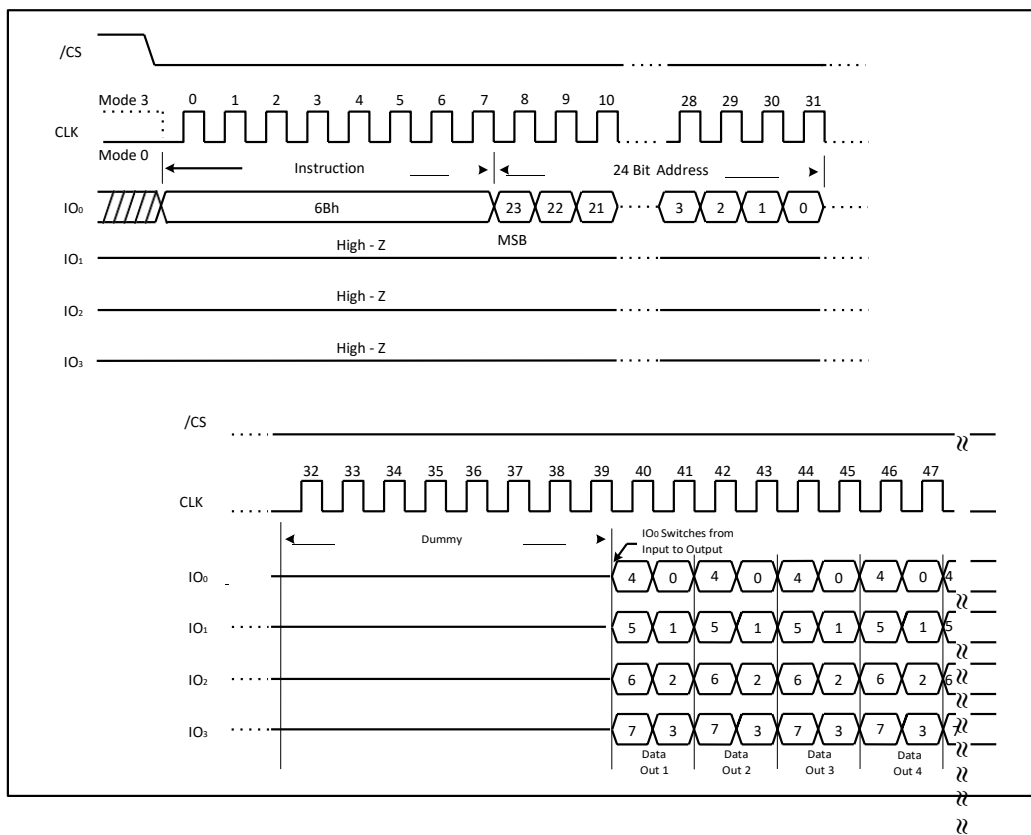
Figure 15. Fast Read Quad Output instruction (SPI Mode)
