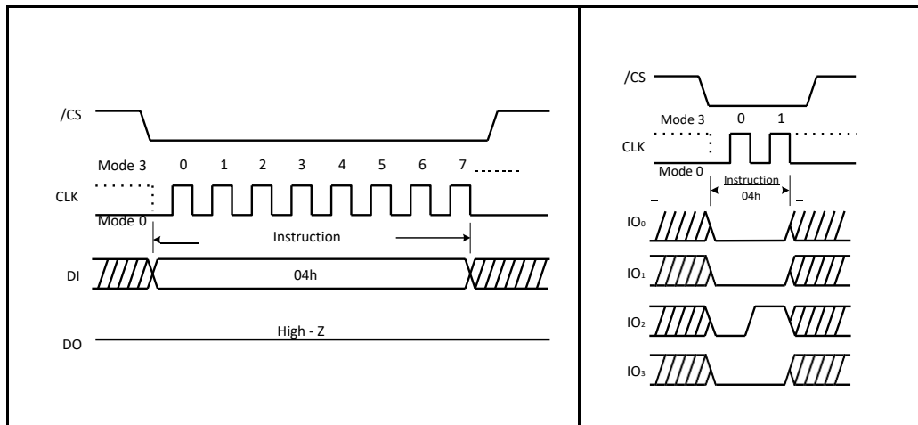
Figure 8. Write Disable Instruction for SPI Mode (left) and QPI Mode (right)
