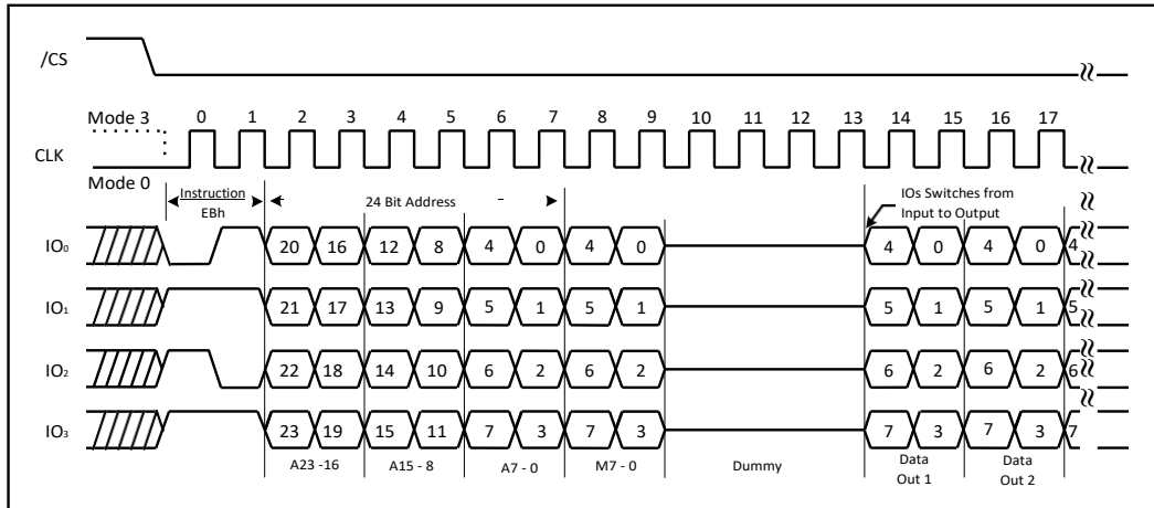
Figure 17d. Fast Read Quad I/O Instruction (Initial instruction or previous M7-0 ≠ Axx, QPI mode, 108MHz)
