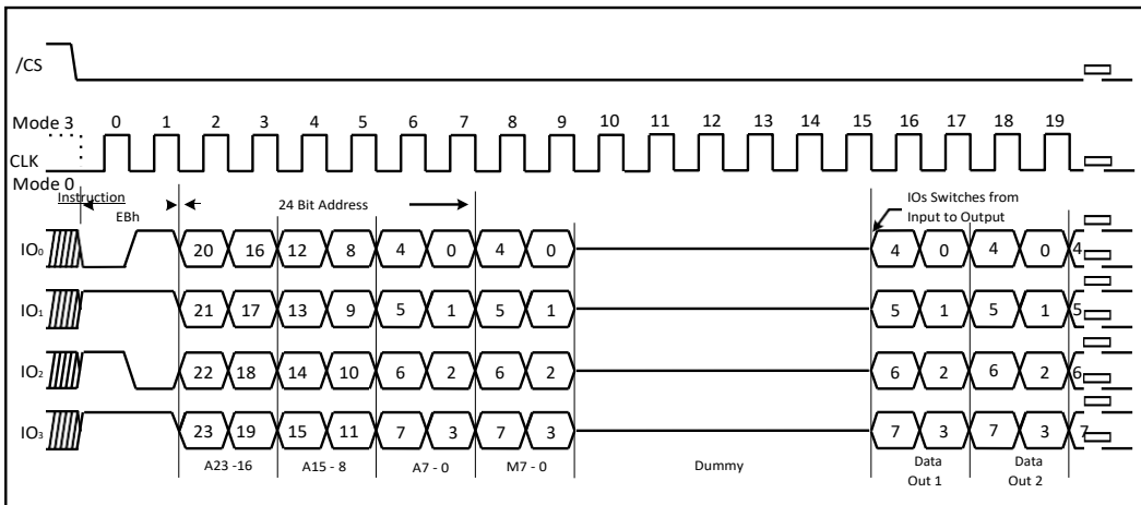
Figure 17e. Fast Read Quad I/O Instruction (Initial instruction or previous M7-0 ≠ Axx, QPI mode, 133MHz)
