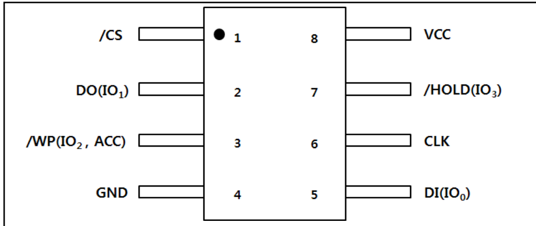
Figure 1a. Pin Assignments, 8-pin SOP 200-mil
