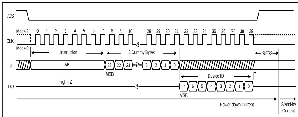
Figure 27c. Release power-down / Device ID Instruction (SPI Mode)
