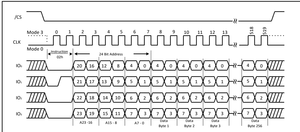
Figure 18b. Page Program Instruction (QPI Mode)
