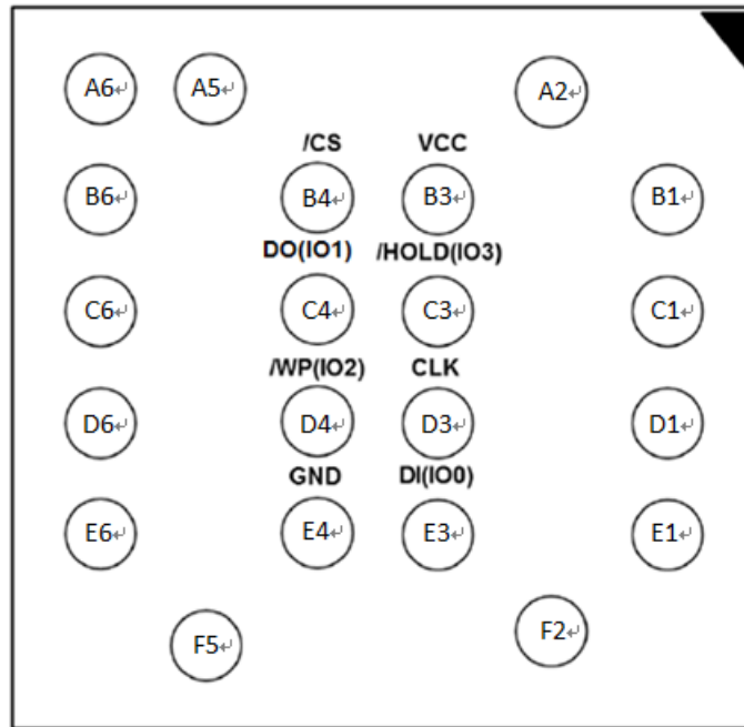
Figure 1c. Pin Assignments,21-Ball WLCSP 0.275mm
